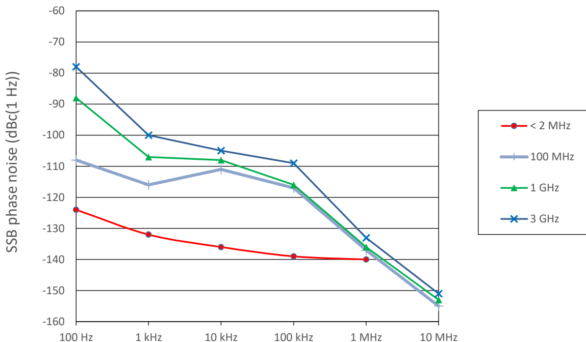
Typical phase noise at different center frequencies.
